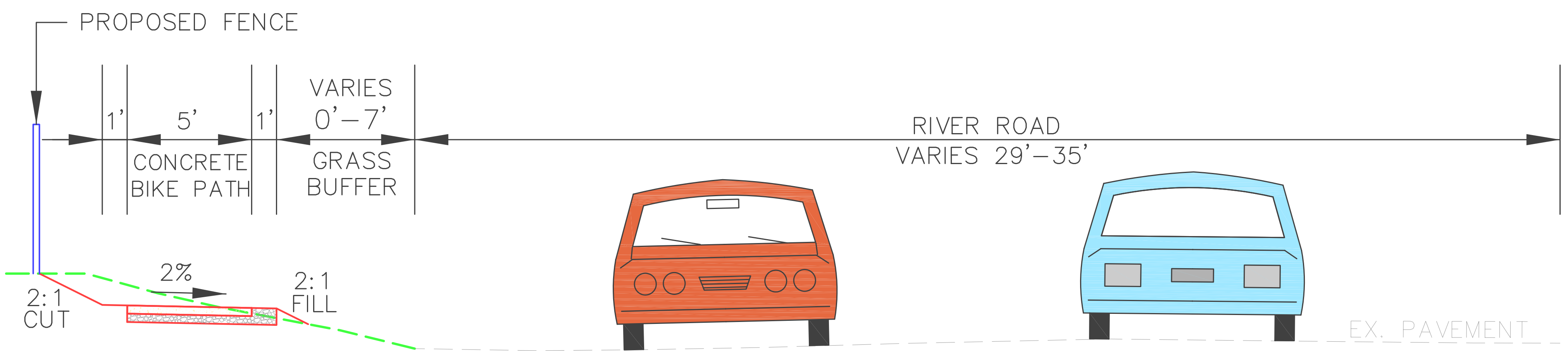
C. STATION 11+00 TO STATION 12+46
