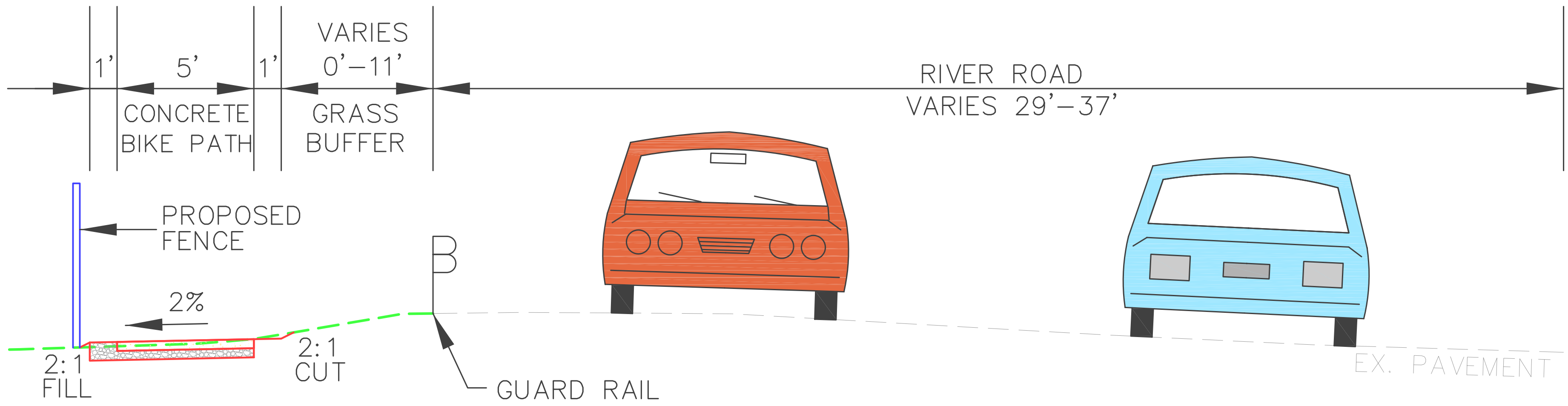
B. STATION 1+14 TO STATION 11+00
