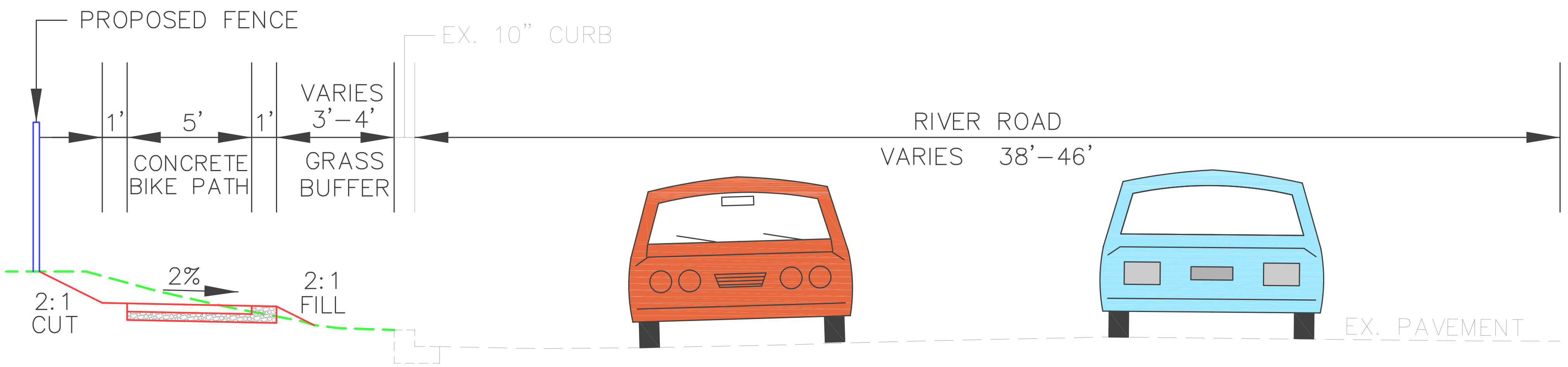
A. STATION 0+34 TO STATION 1+14
